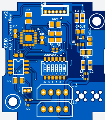
CS10-CM07 – Bottom view of the PCB board.
