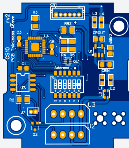
CS10-CM03 – Bottom view of the PCB board.
