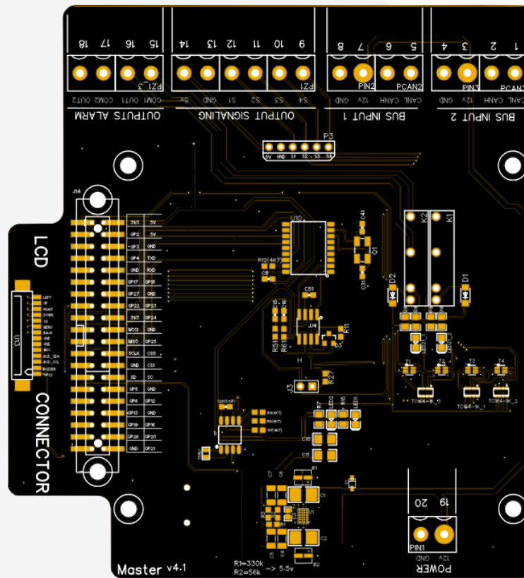
CS10-CP01 - Bottom view of the PCB board.
